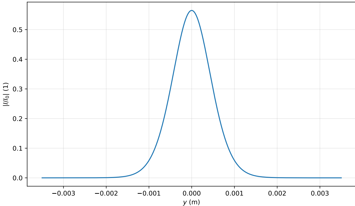
Intensity profile I(x=0, y, z=2.627)/I_0 , P_{in}=0.4P_{cr} , artificial time
